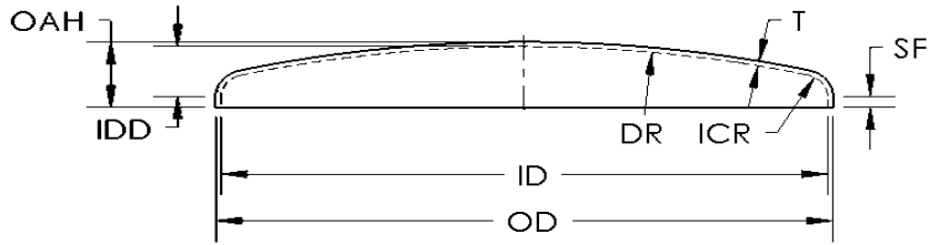
STANDARD, SHALLOW NON-CODE FLANGED & DISHED 28" to 84" 3/16" to 5/8"
