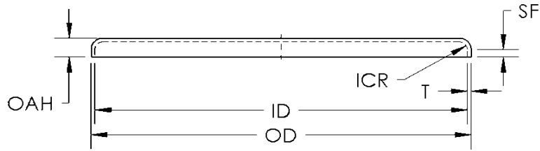
FLANGED ONLY 28" to 84" 3/16" to 1/2"
