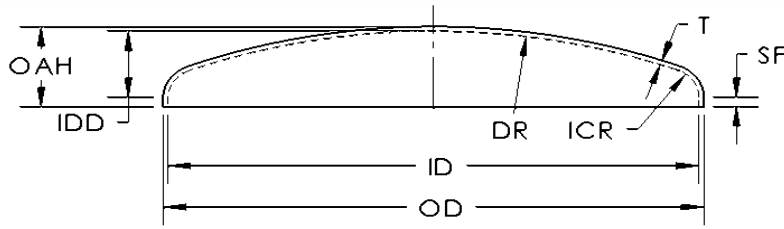
STANDARD, NON-CODE FLANGED & DISHED 28" to 84" 3/16" to 5/8"
