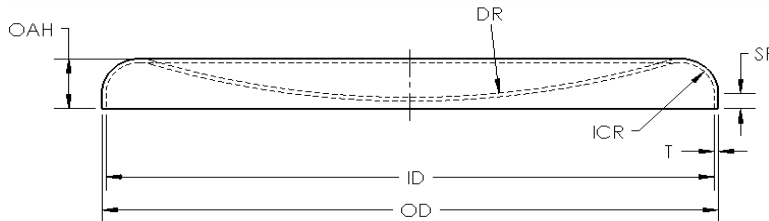
FLANGED & REVERSE DISHED 28" to 84" 3/16" to 1/2" DR = OD X 1.4
