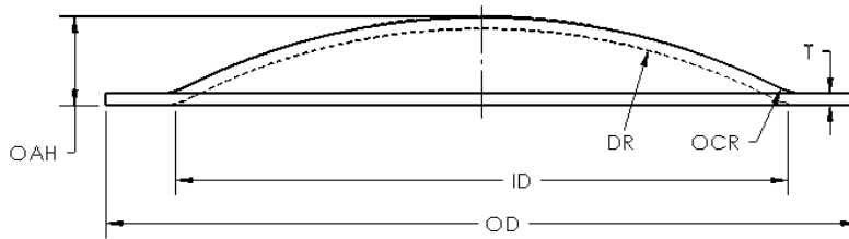
FLARED & DISHED 20.00"ID to 48.00"ID
